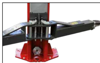
Rubber door protections. Toothed sector arm rotation stop system.
